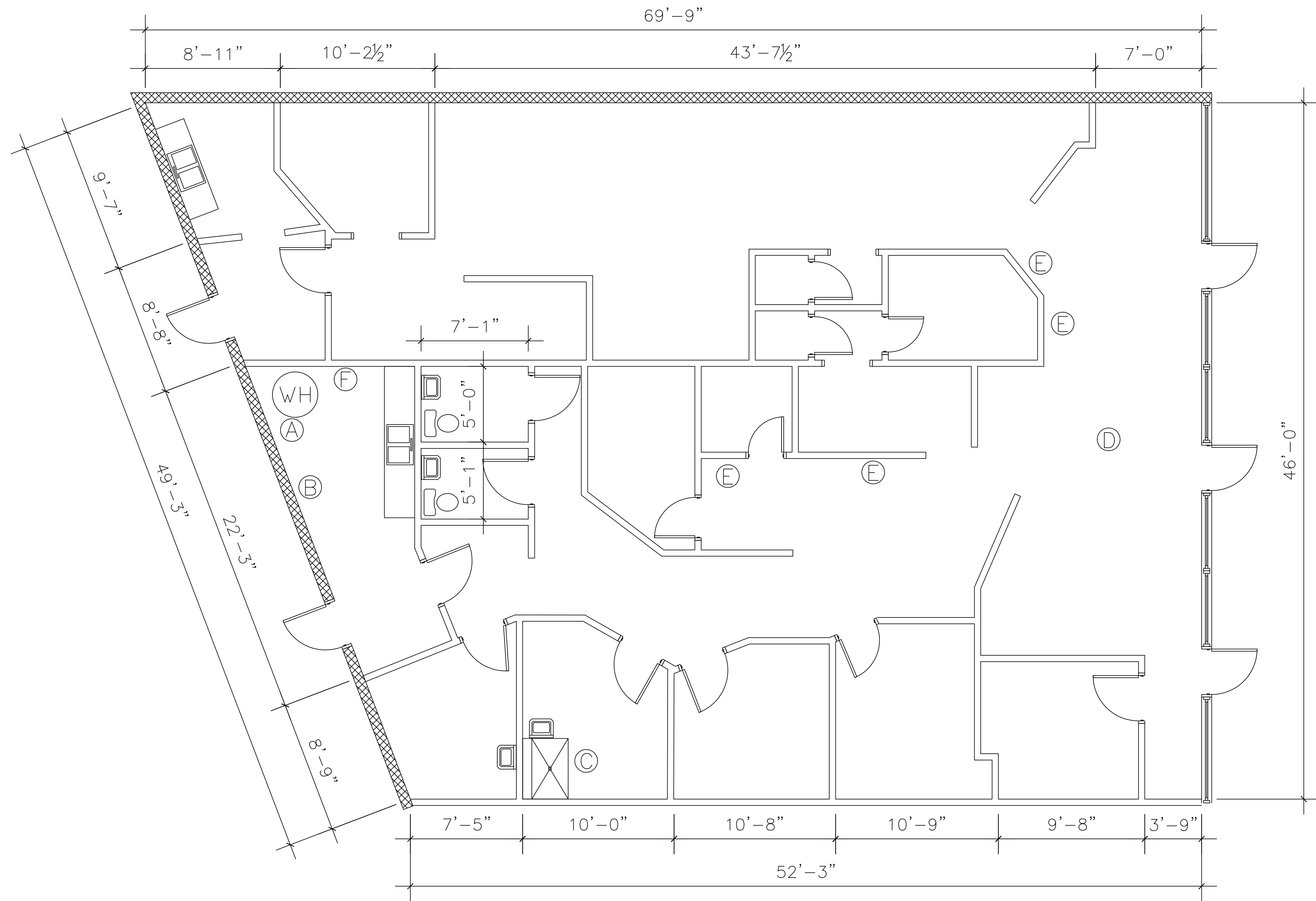
EXISTING FLOORPLAN: SCALE: 1/4" = 1'
