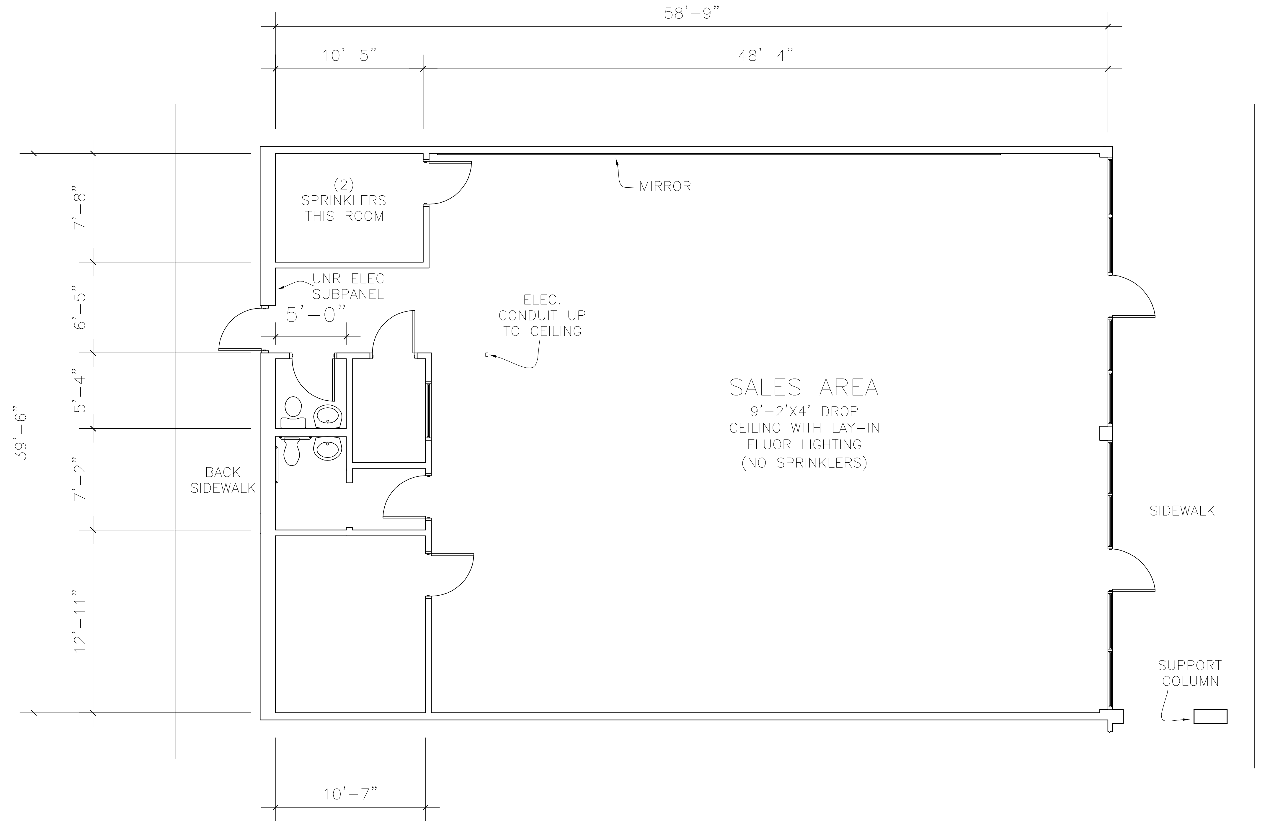
EXISTING FLOOR PLAN: SCALE: 1/4" = 1'
