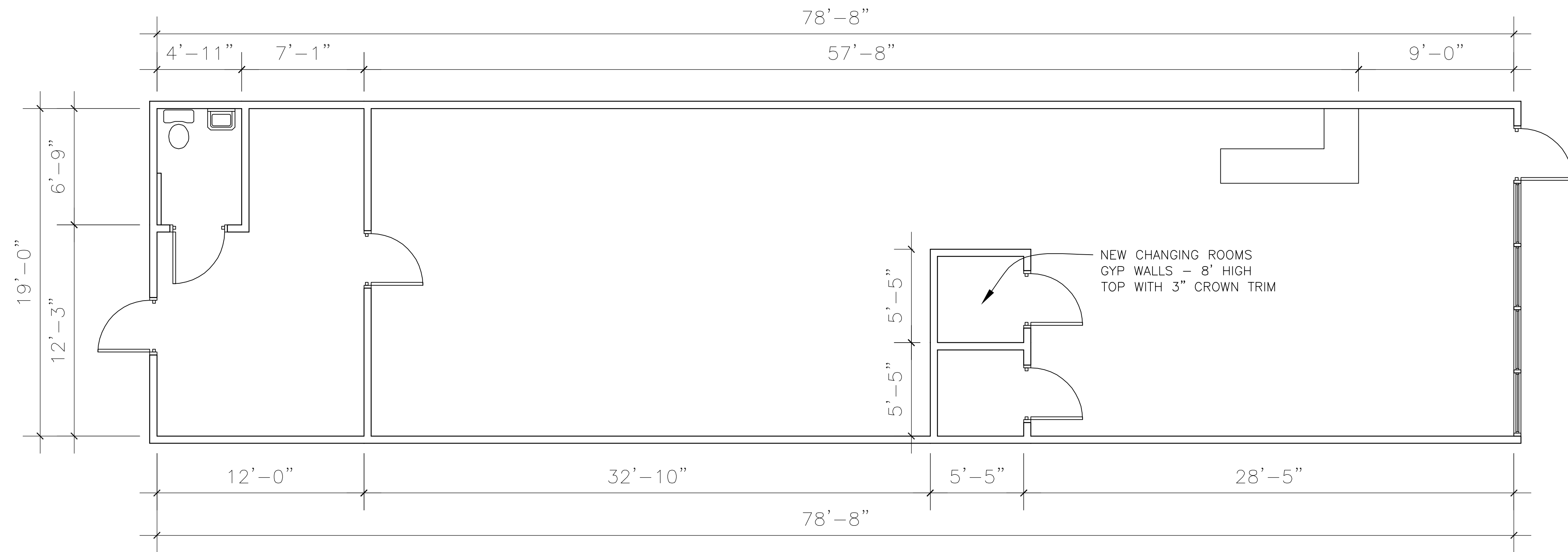
EXISTING FLOORPLAN: SCALE: 1/4" = 1'
